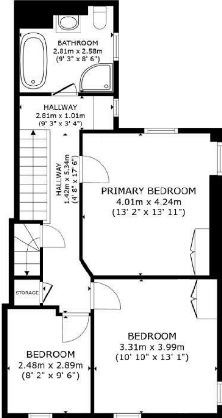
FLOOR 2
